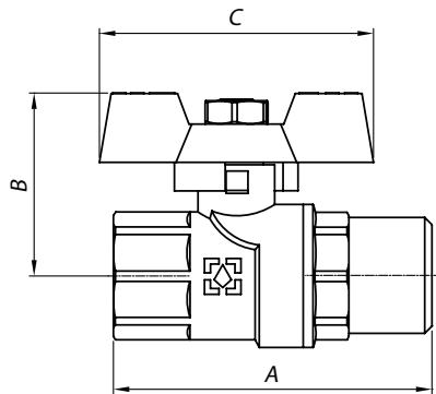
Ball valve with T-handle series Yellow (MF)
