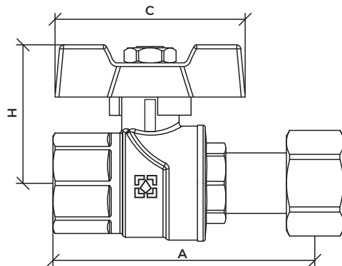
Ball valve straight with connectors series Black
